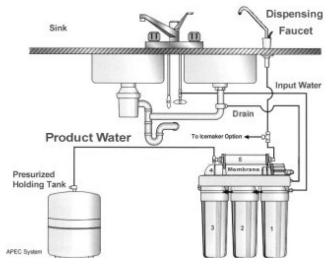
Standard reverse osmosis system
